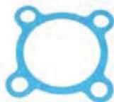
SK-17-40005-05-AM GASKET SUCTION 4 BOLT
